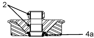
(3d) Wiping Stem Seal Adapter
